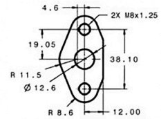
Oil Inlet
